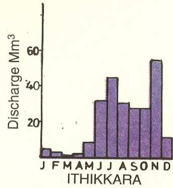
MEAN MONTHLY DISCHARGE (1978 - 82)
